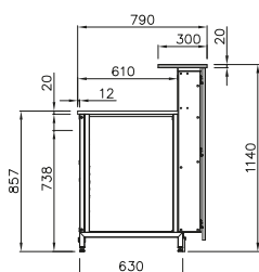
BAELSN balcão slim neutro dry/ambient slim line bar counter comptoir slim neutre barra slim neutra
