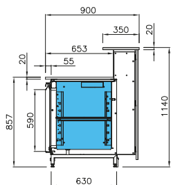
BAELR 3M1 balcão refrigerado refrigerated counter comptoir réfrigéré barra refrigerada
