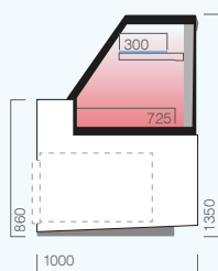
VDS AQV - VD H1350 aquecida ventilada heated ventilated DIM. 1250 | 1875*
