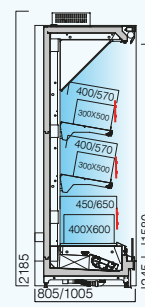
MF2 700/900 PF CC - SG
