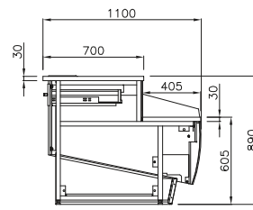
PACS 2N caixa support counter caisse caja
