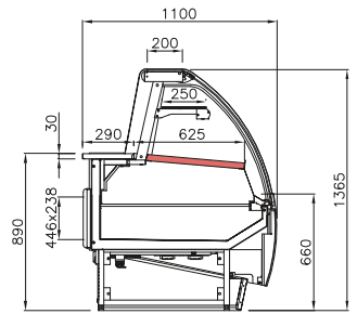
PATA tampo aquecido heated deck plateau chaud tampo caliente
