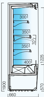
MPRT mural multideck 3M1 (-1... +5 °C) DIM. 680 | 980 | 1280 1480 | 1880
